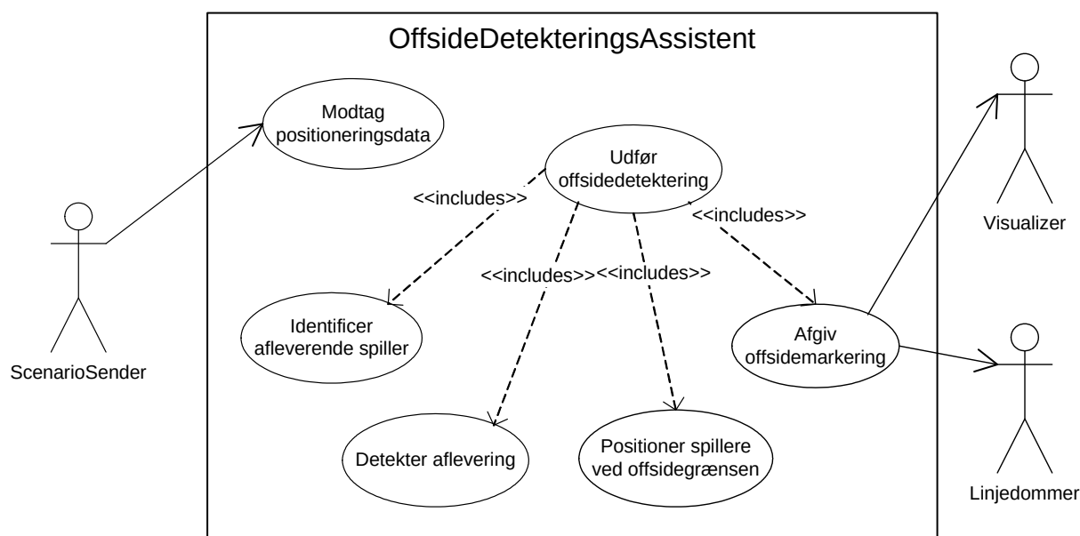
Figur 48 – Use Case-diagram for ODA.
