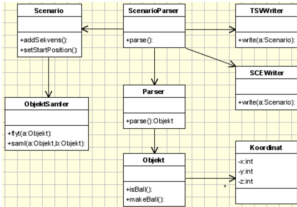
Figur 59 – Klassediagram for ScenarioGenerator.
